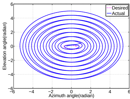
Fig. 11 Spiral motion
